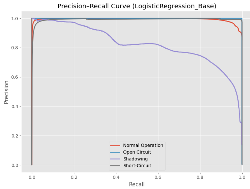
Figure 21: Logistic Regression: Precision-Recall Curve
