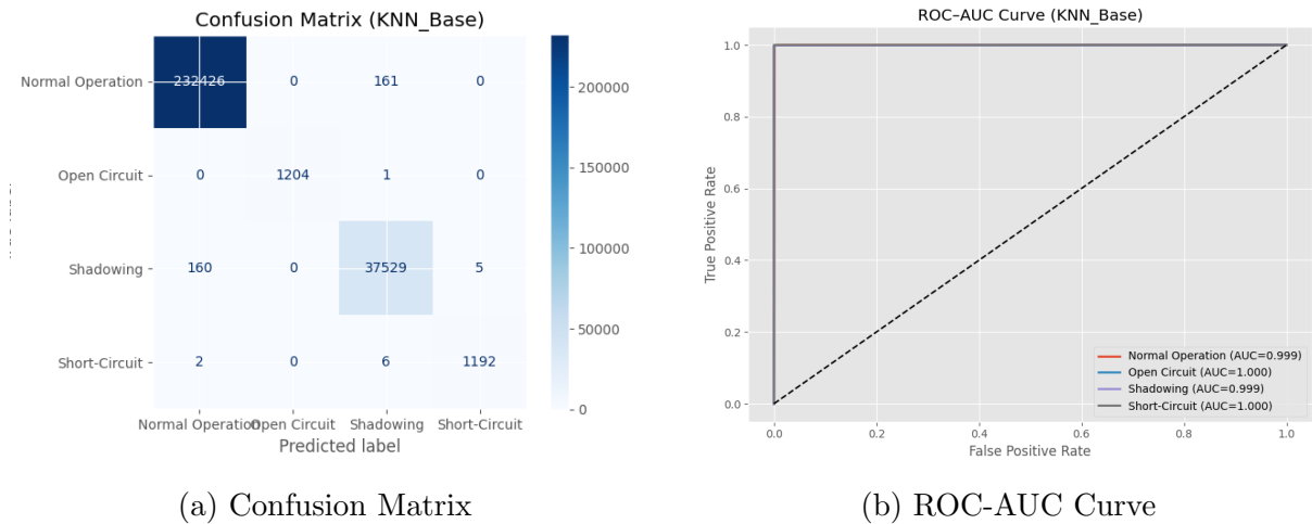
Figure 12: KNN: Classification Performance
