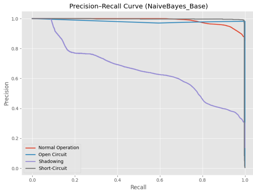
Figure 15: Naive Bayes: Precision-Recall Curve
