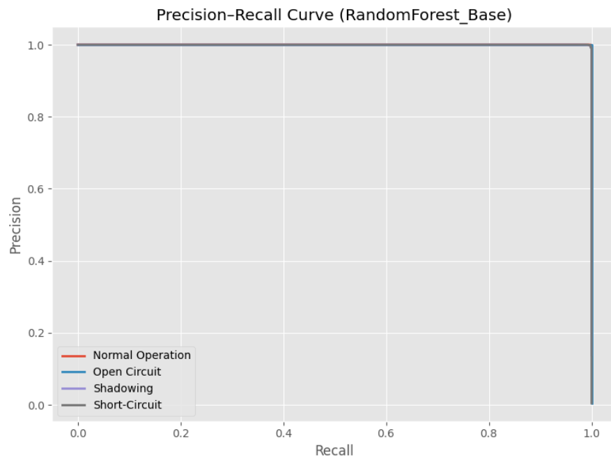
Figure 17: Random Forest: Precision-Recall Curve
