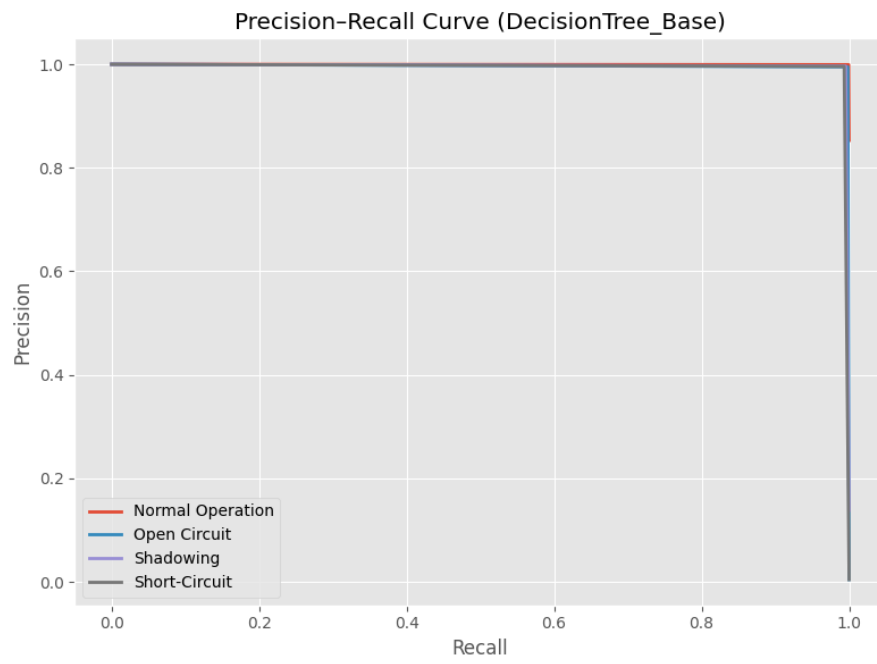
Figure 23: Decision Tree: Precision–Recall Curve
